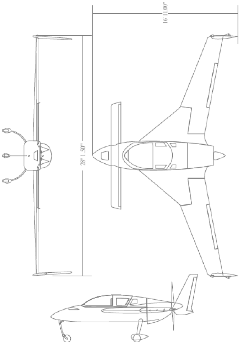
Figure 1: Cozy MKIV 3-View
