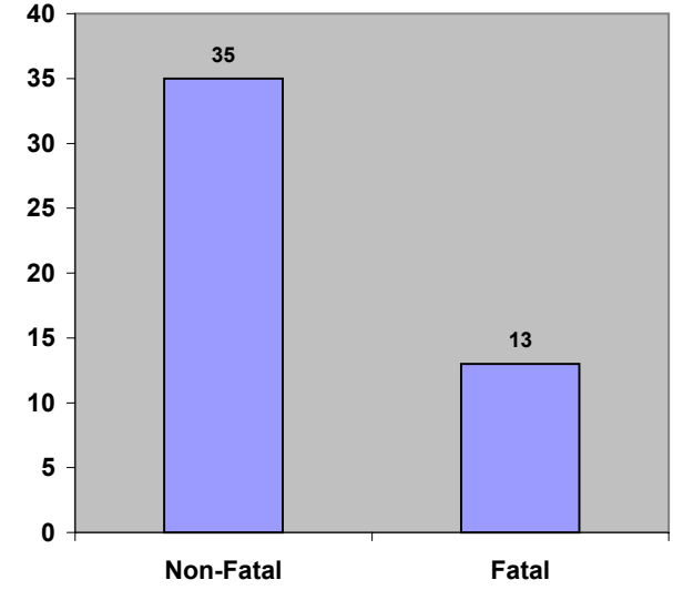
Severity Count
