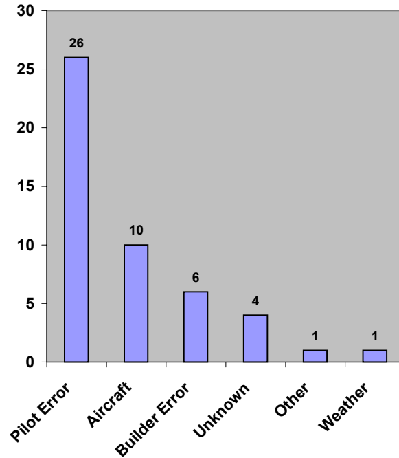
Category Count
