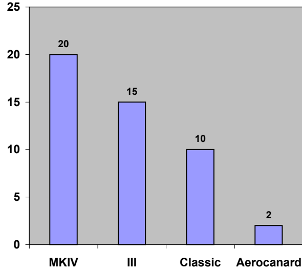
Type Count
