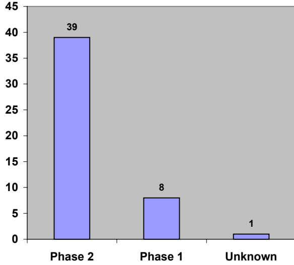
Phase Count
