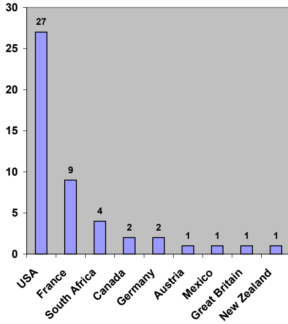
Country Count
